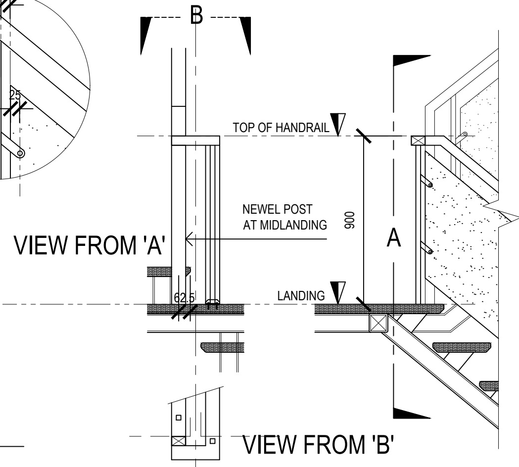
PENTHOUSE RAILINGS DETAILS AT LANDING SCALE 1:20
