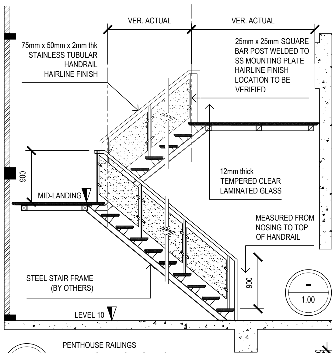
PENTHOUSE RAILINGS GLASS SECTION ALONG STEPS TYP. SCALE 1:20
