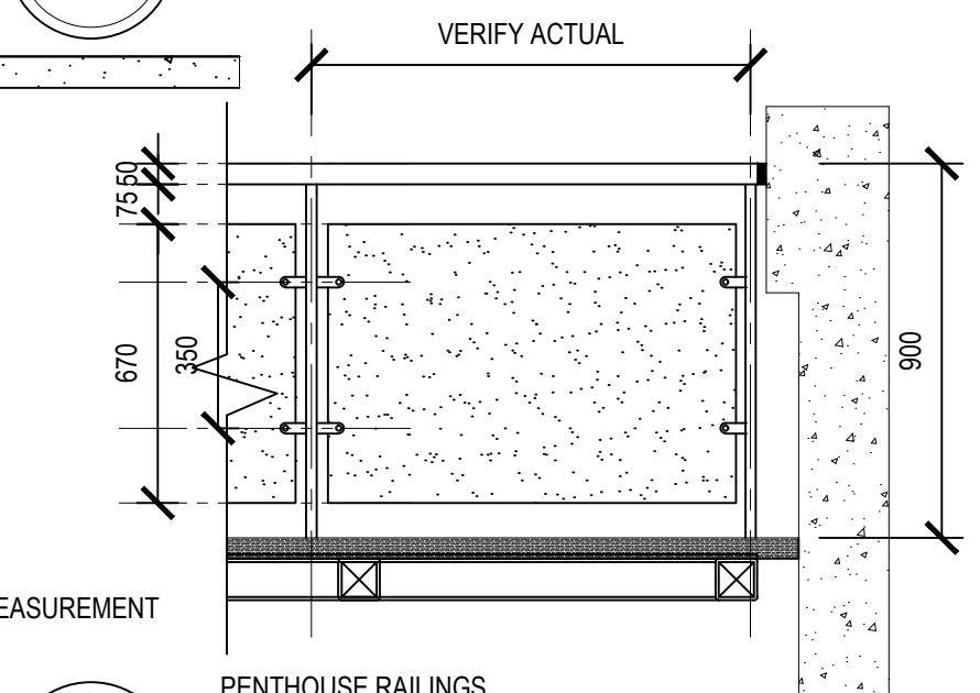
PENTHOUSE RAILINGS GLASS SECTION AT LANDING TYP. SCALE 1:20
